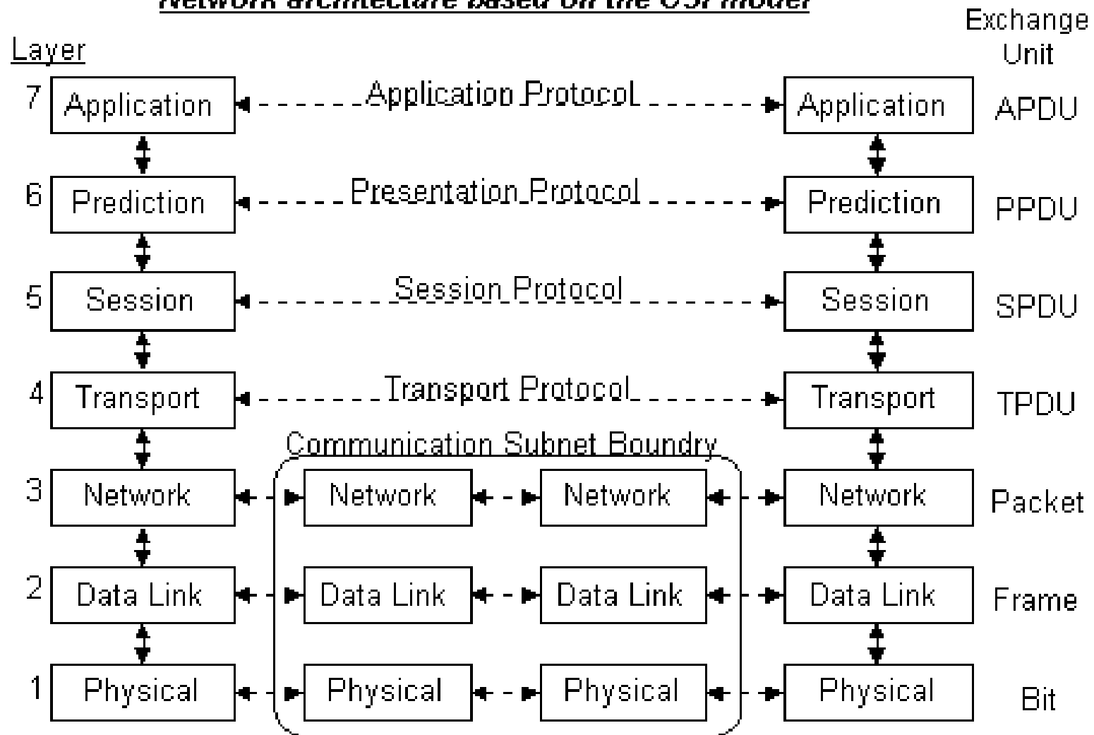
Network architecture based on the OSI model
