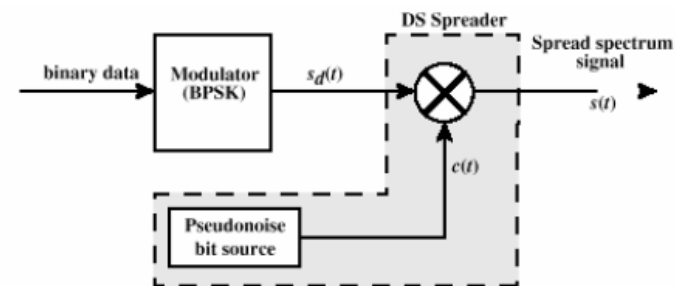
(a) Transmitter
